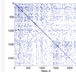
(e) yeast
