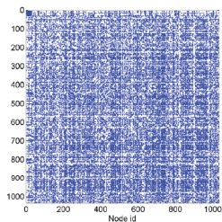
(a) facebook107
