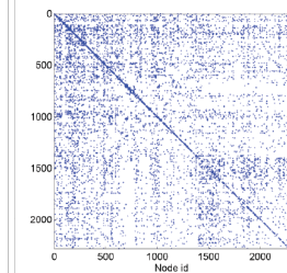
(e) yeast
