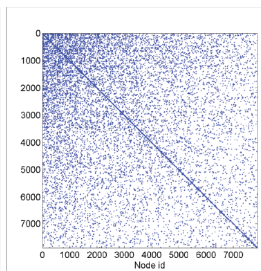
(i) cond-mat2
