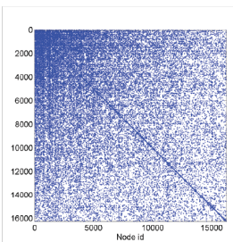
(h) cond-mat1
