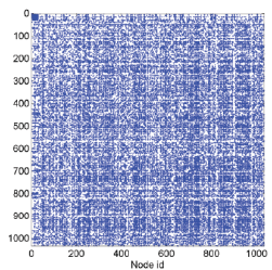
(a) facebook107
